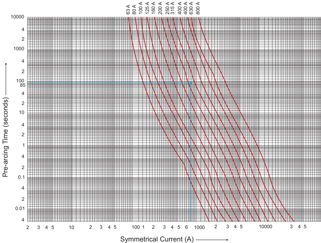
Time-Current Characteristics
